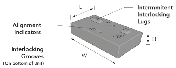
CLOSED END/CORNER 17.75 X 3.35 X 10.25 451 MM X 89 MM X 260 MM
